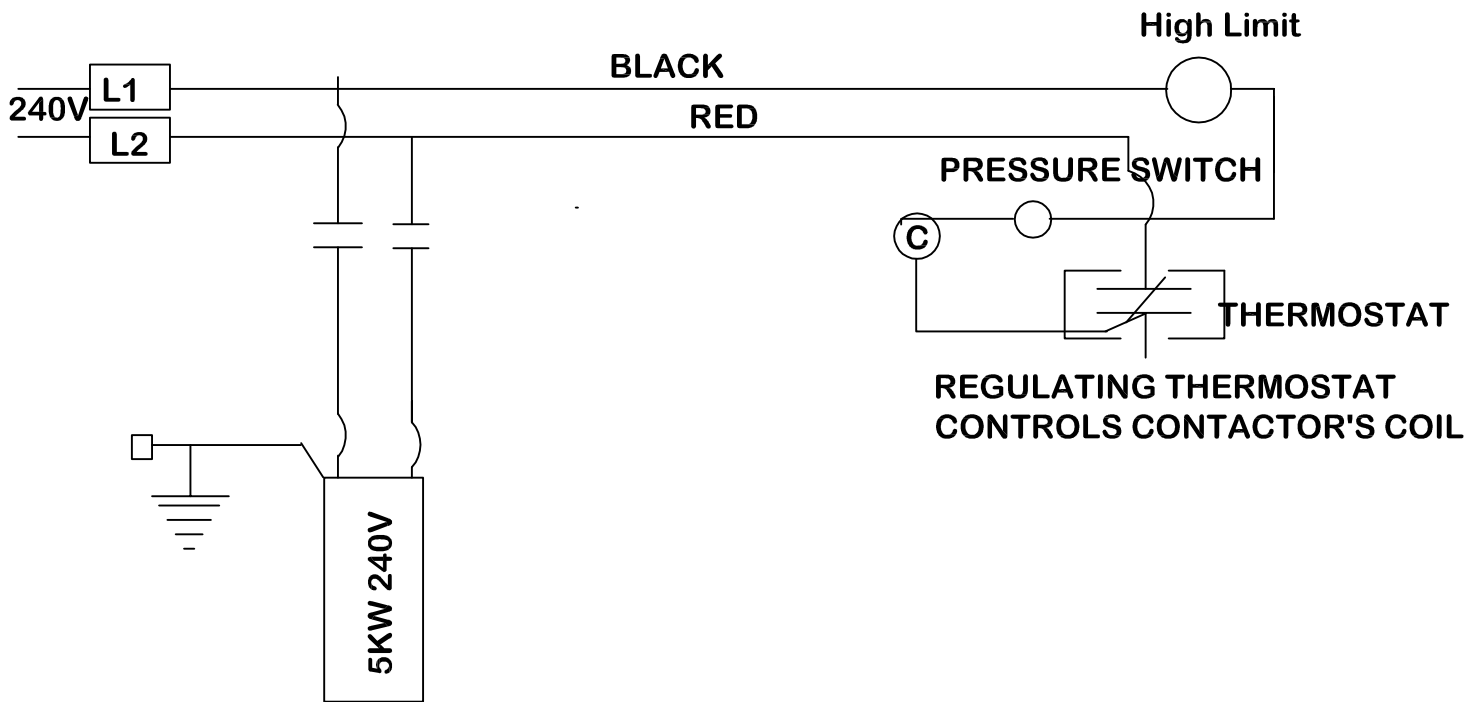
K5 5KW HEATER 240 V
