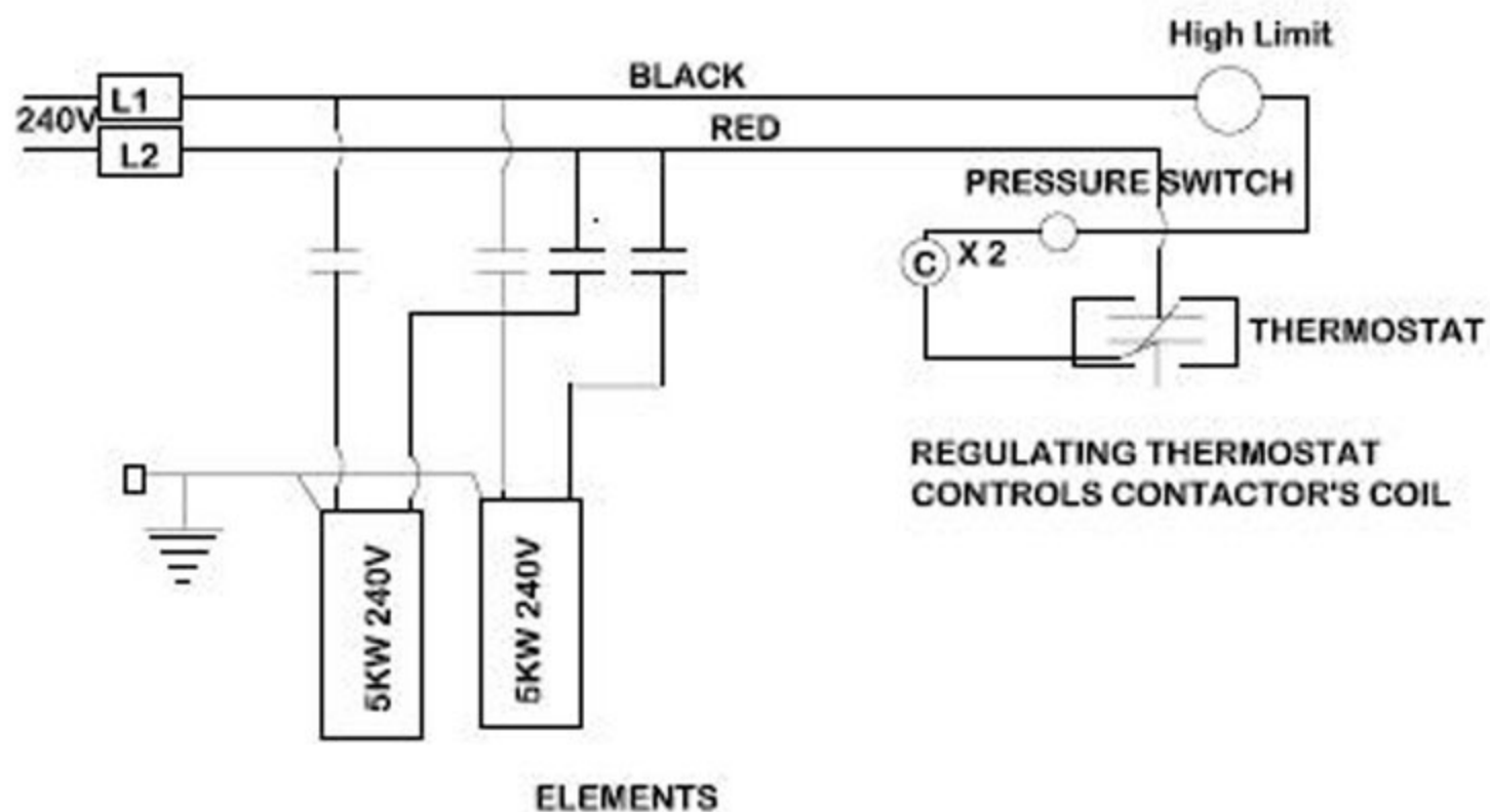
K10 10KW HEATER 240 V
